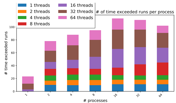
Figure 2. Number of time exceeded runs per process.
