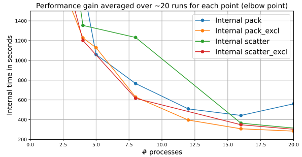
Figure 6. Processes and time execution runs elbow point.
