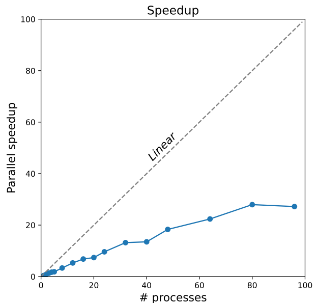
Figure 7. Speedup
