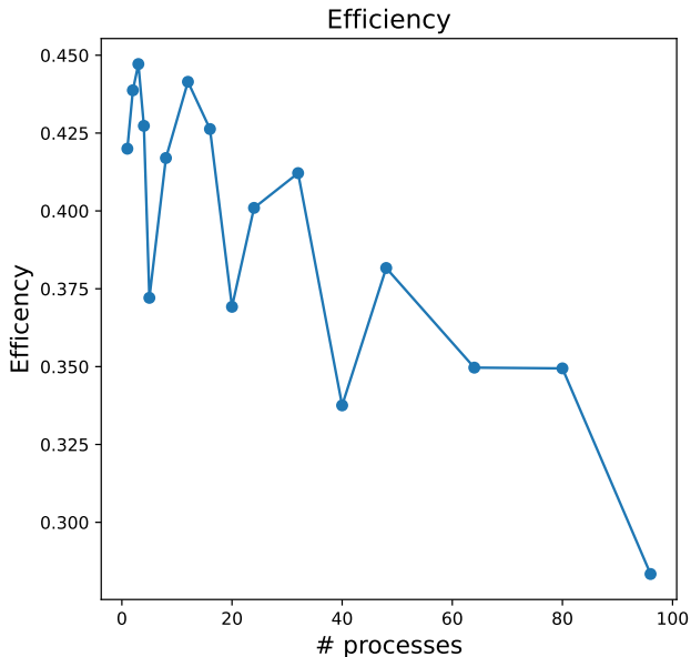
Figure 8. Efficiency
